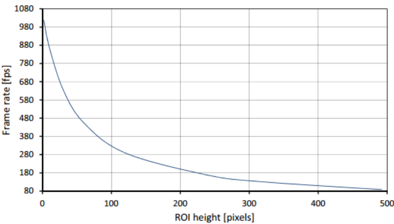
Figure 9: Frame rate as a function of ROI height
